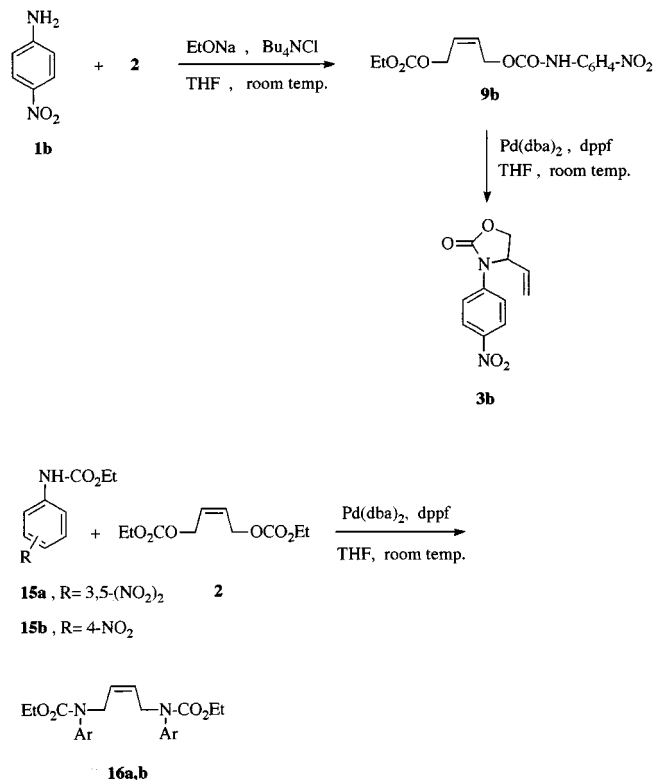
Scheme 5. Complementary experiments
