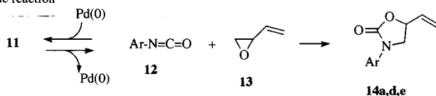
Scheme 4. Sequence of events leading to N -aryloxazolidin-2-ones 3 and 14
