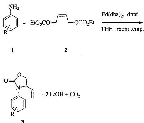
Scheme 2. Pd 0 -catalyzed formation of N -aryl-4-vinylloxazolidin-2-ones
